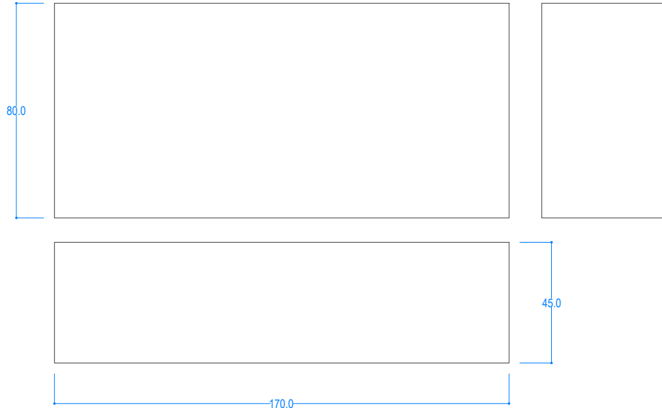
PEANYA 22 VISTA FRONTAL, LATERAL I PLANTA
