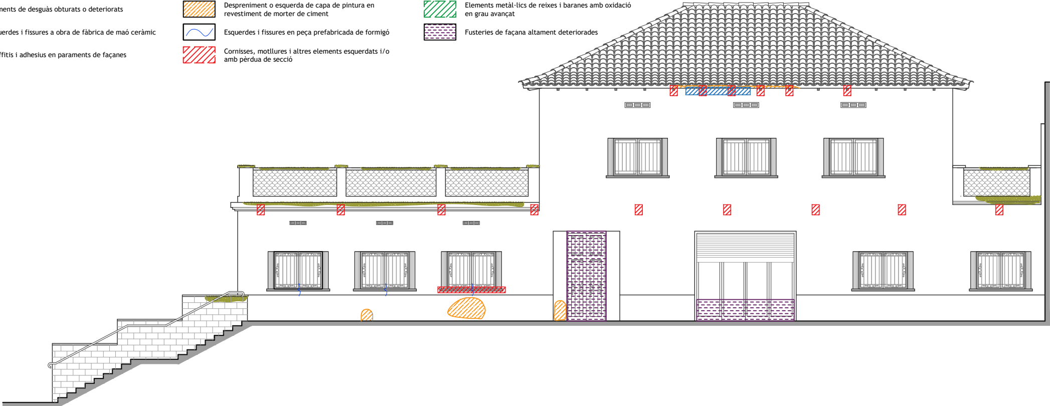
FAÇANA PRINCIPAL
